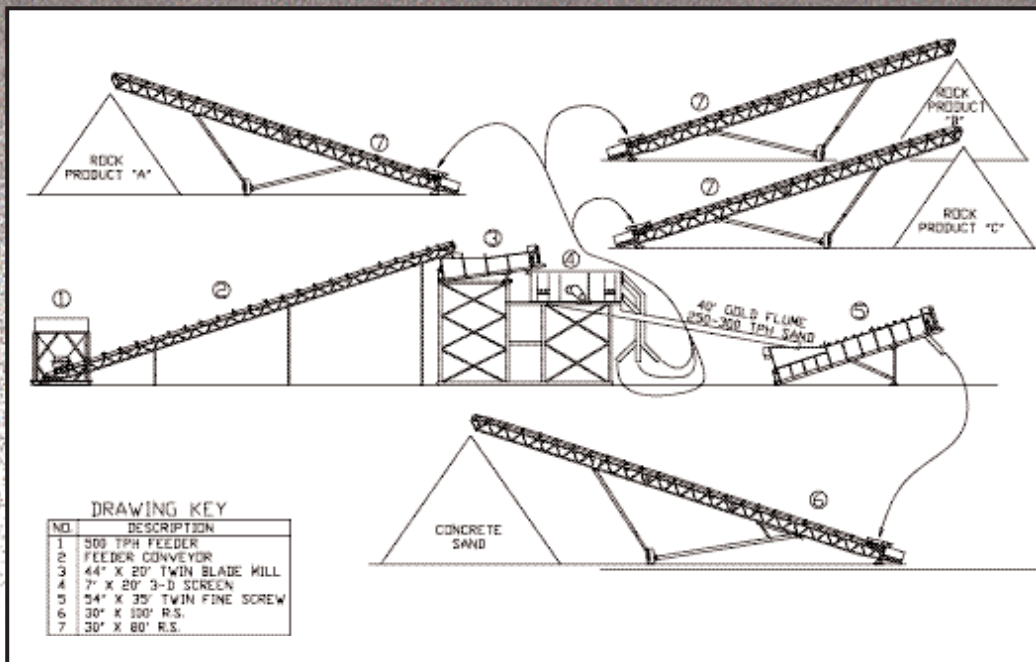
CAD DRAWING OF A TYPICAL PLANT LAYOUT USING QUALITY GREYSTONE EQUIPMENT
